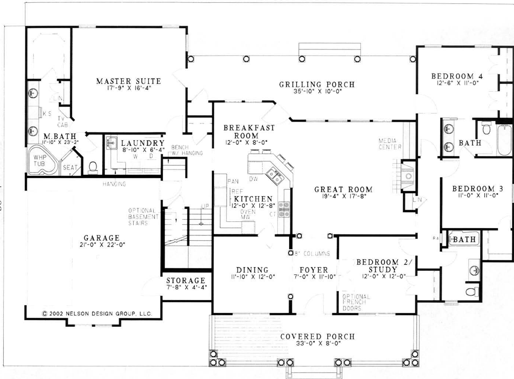
Main Floor
